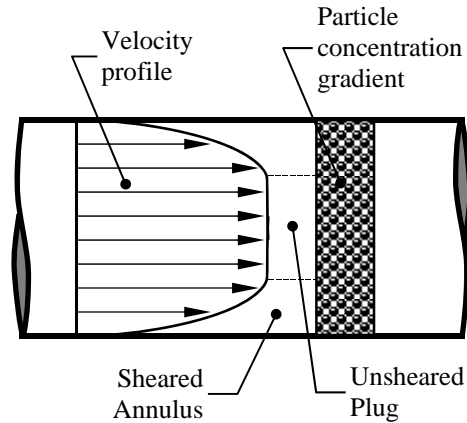
Figure 2. Homogeneous laminar flow
